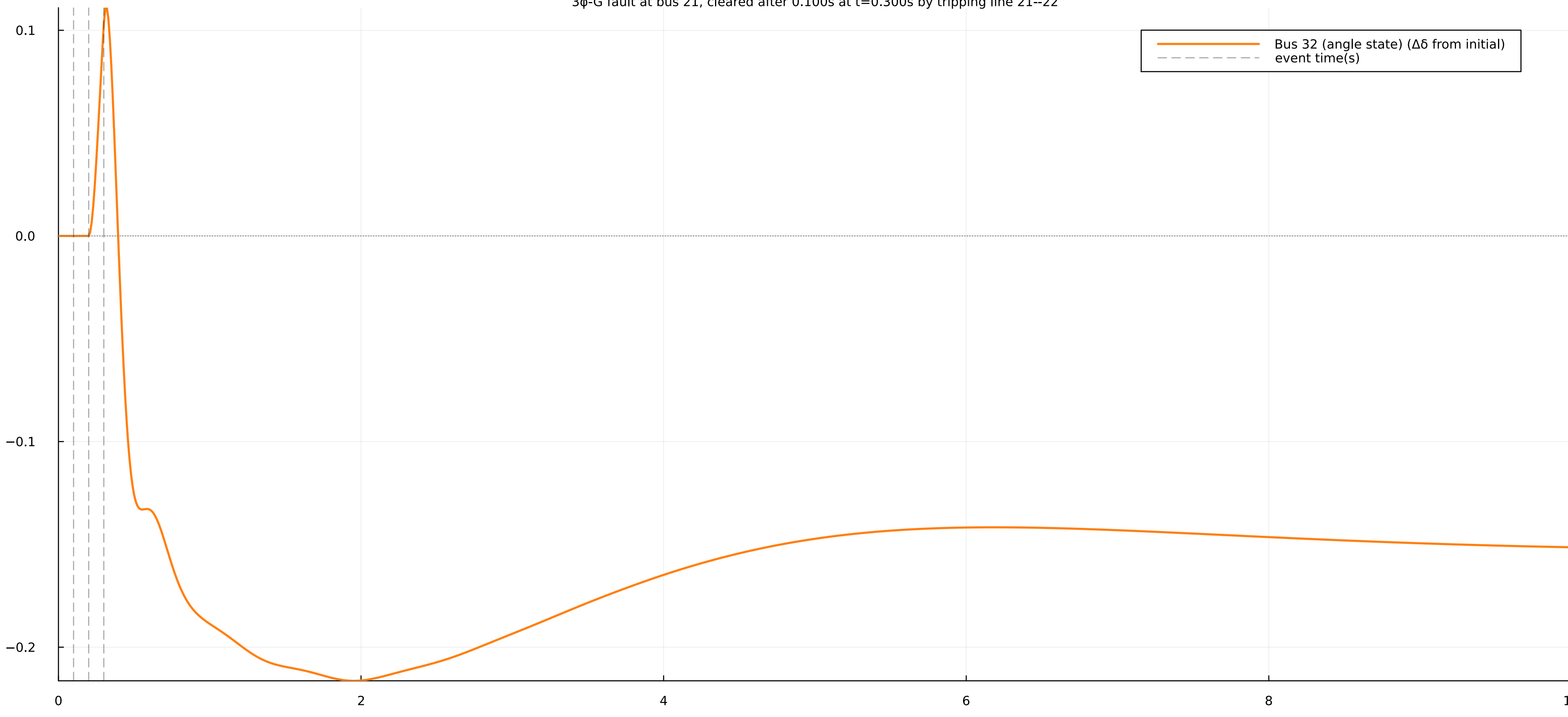
Rotor/angle deviation at bus 32 3φ-G fault at bus 21, cleared after 0.100s at t=0.300s by tripping line 21--22
