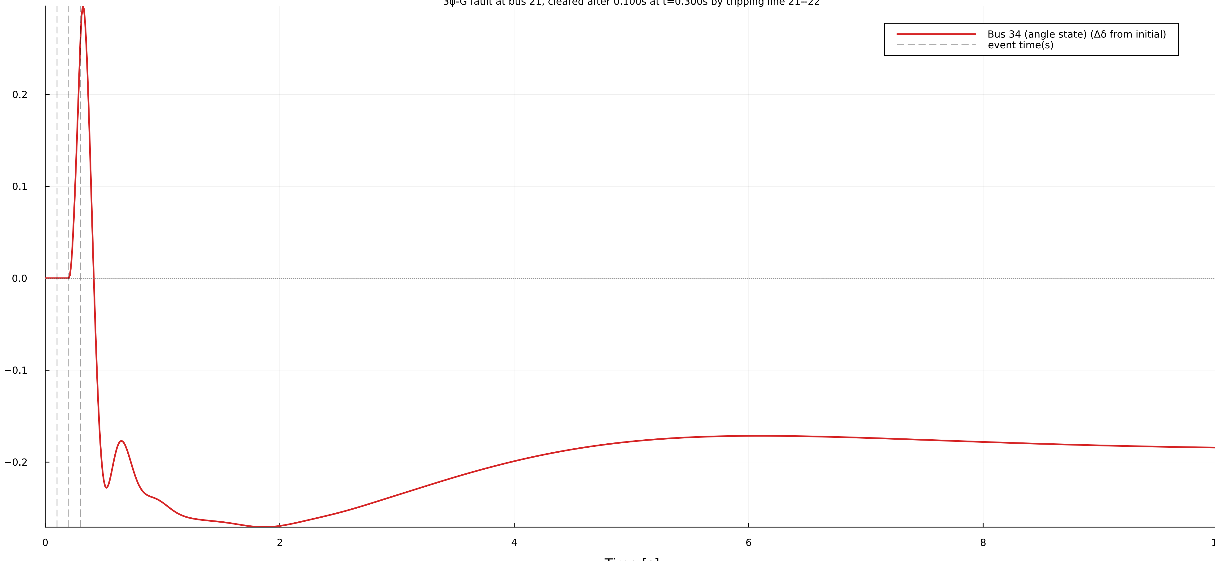
Rotor/angle deviation at bus 34 3φ-G fault at bus 21, cleared after 0.100s at t=0.300s by tripping line 21--22
