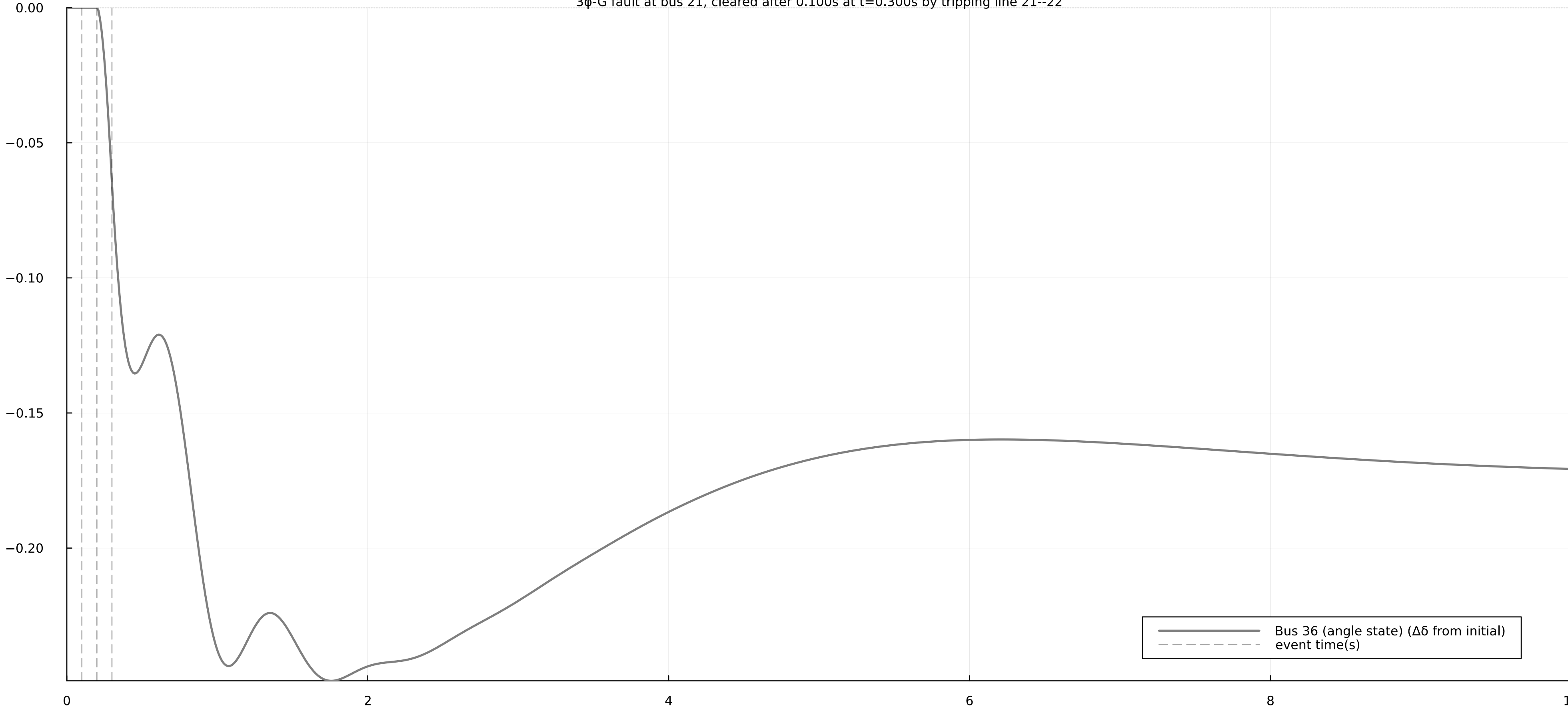
Rotor/angle deviation at bus 36 3 \phi -G fault at bus 21, cleared after 0.100s at t=0.300s by tripping line 21--22
