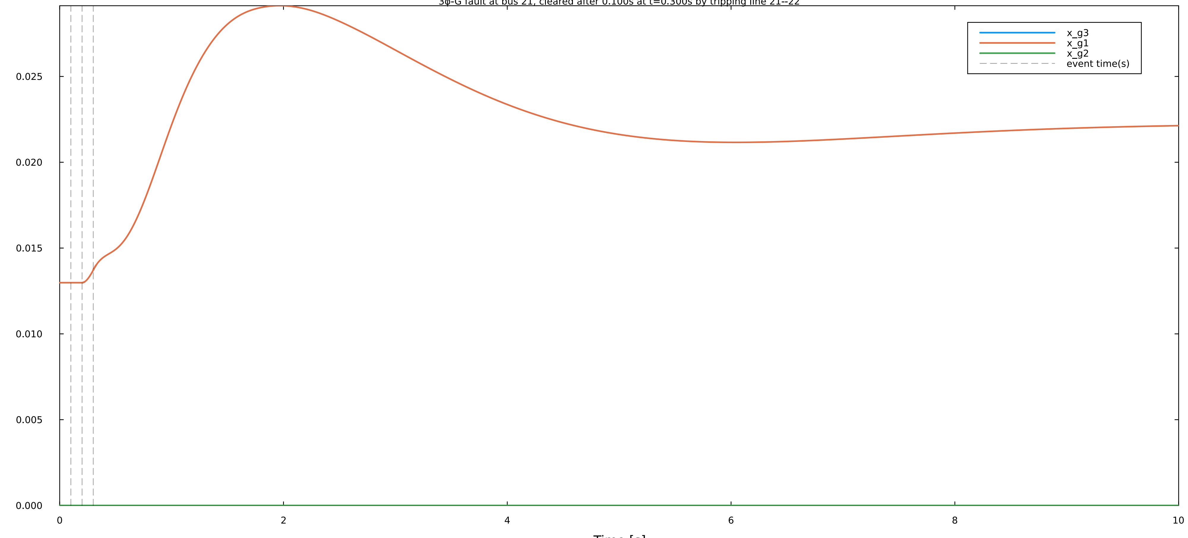
TGType1 states at bus 39 3φ-G fault at bus 21, cleared after 0.100s at t=0.300s by tripping line 21--22
