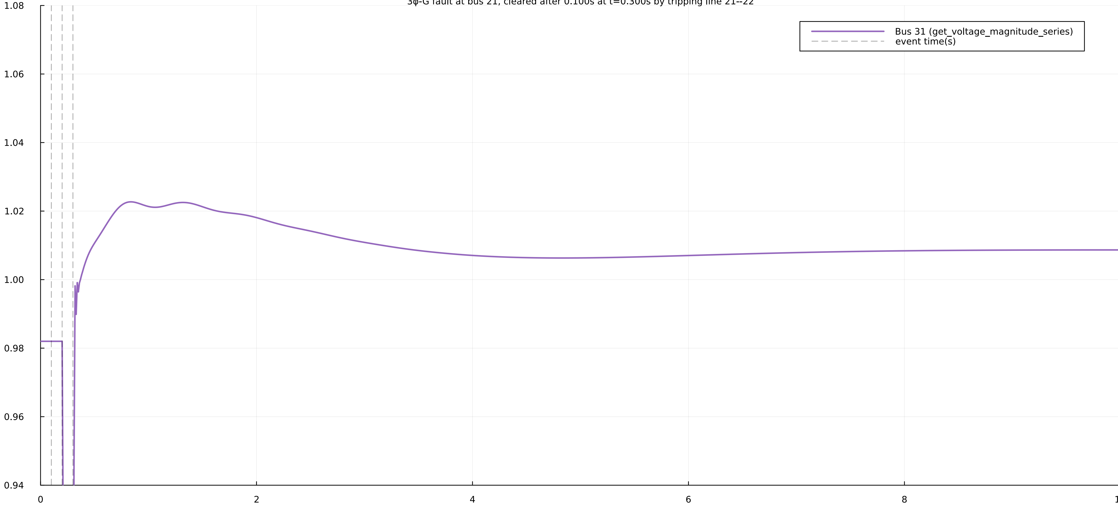
Voltage magnitude at bus 31 [V0=0.9820 pu] 3φ-G fault at bus 21, cleared after 0.100s at t=0.300s by tripping line 21--22
