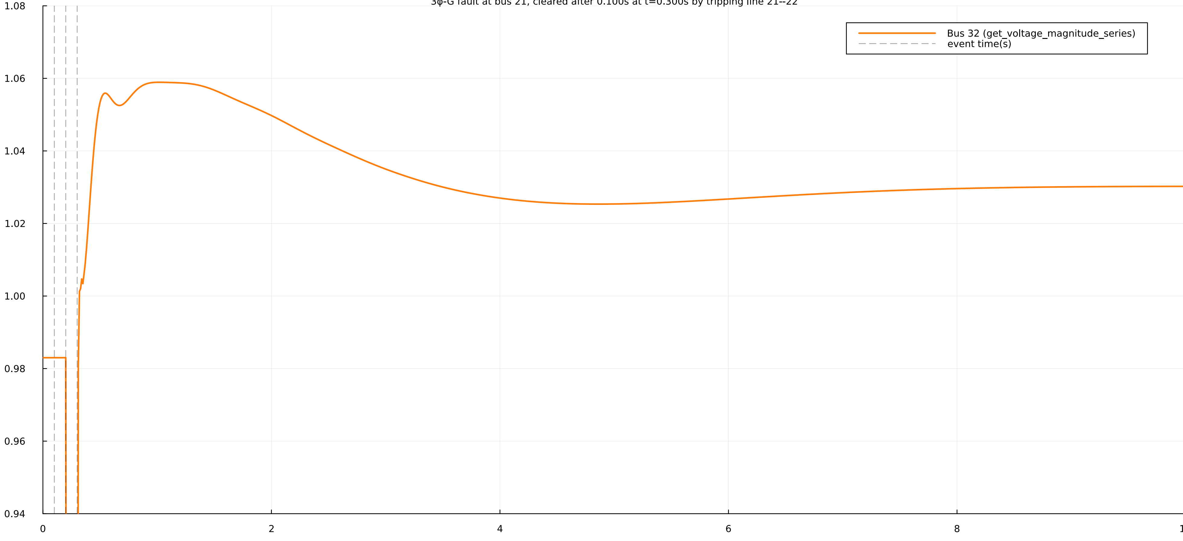
Voltage magnitude at bus 32 [ V_0=0.9830 pu] 3 \phi -G fault at bus 21, cleared after 0.100s at t=0.300s by tripping line 21--22
