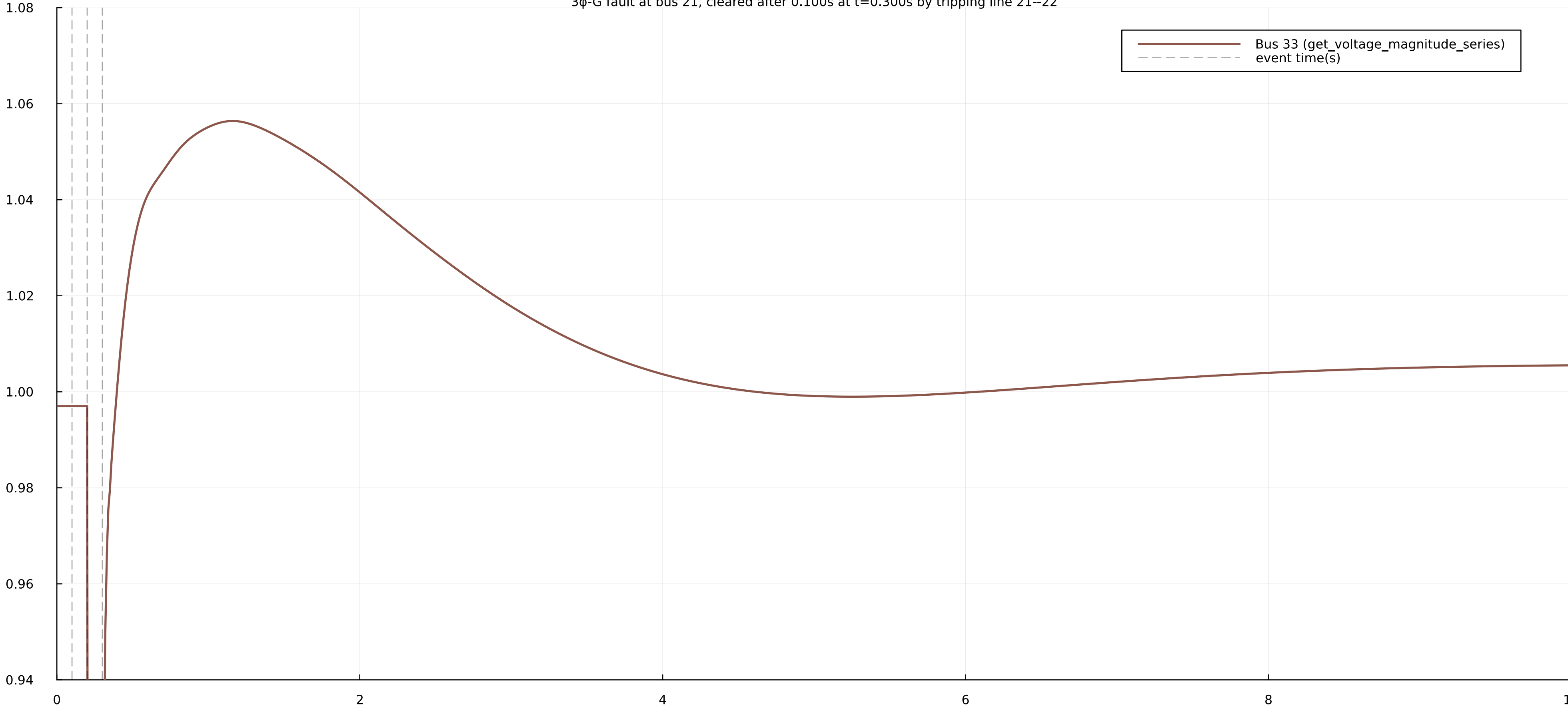
Voltage magnitude at bus 33 [V0=0.9970 pu] 3φ-G fault at bus 21, cleared after 0.100s at t=0.300s by tripping line 21--22
