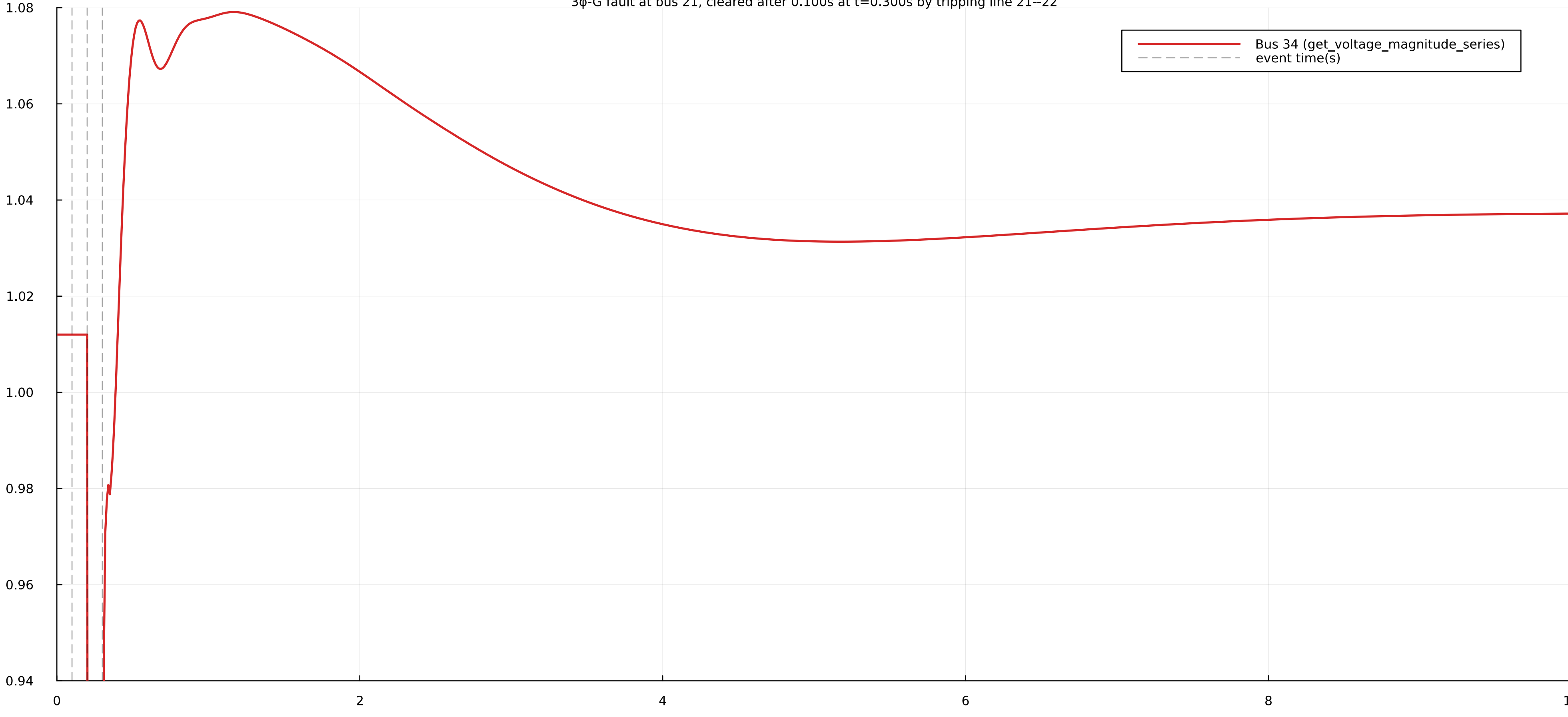
Voltage magnitude at bus 34 [V0=1.0120 pu] 3φ-G fault at bus 21, cleared after 0.100s at t=0.300s by tripping line 21--22
