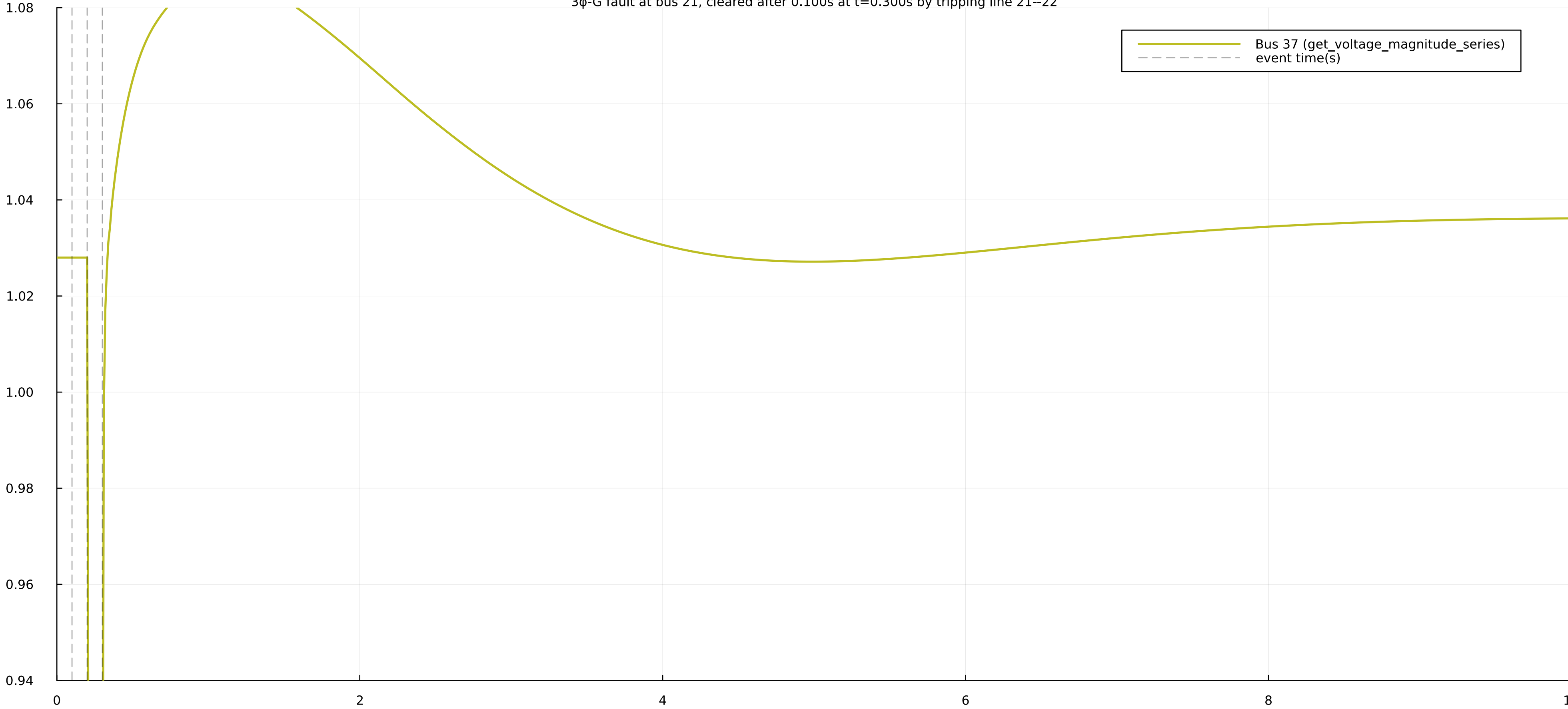
Voltage magnitude at bus 37 [V0=1.0280 pu] 3φ-G fault at bus 21, cleared after 0.100s at t=0.300s by tripping line 21--22
