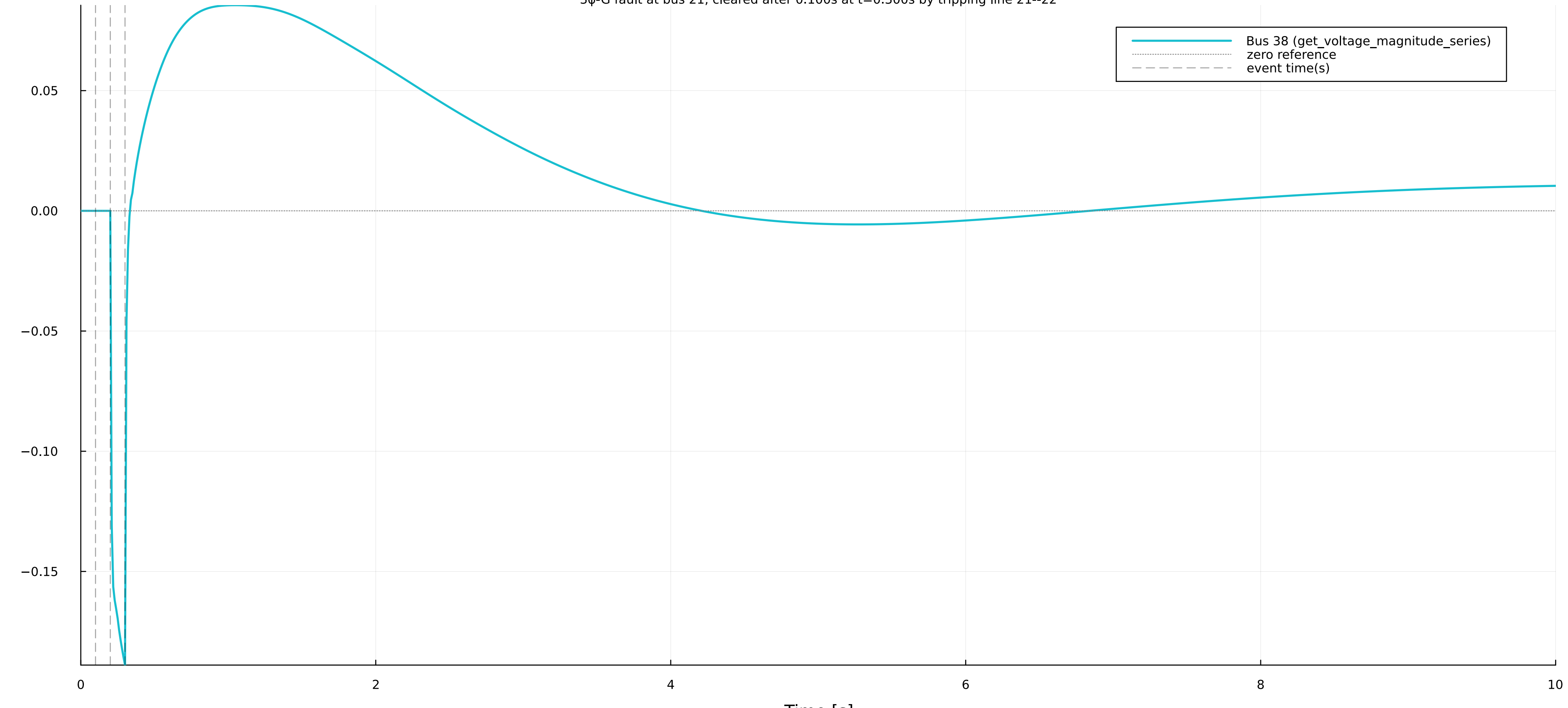
Voltage-magnitude deviation at bus 38 [V0=1.0260 pu] 3 \phi -G fault at bus 21, cleared after 0.100s at t=0.300s by tripping line 21--22
