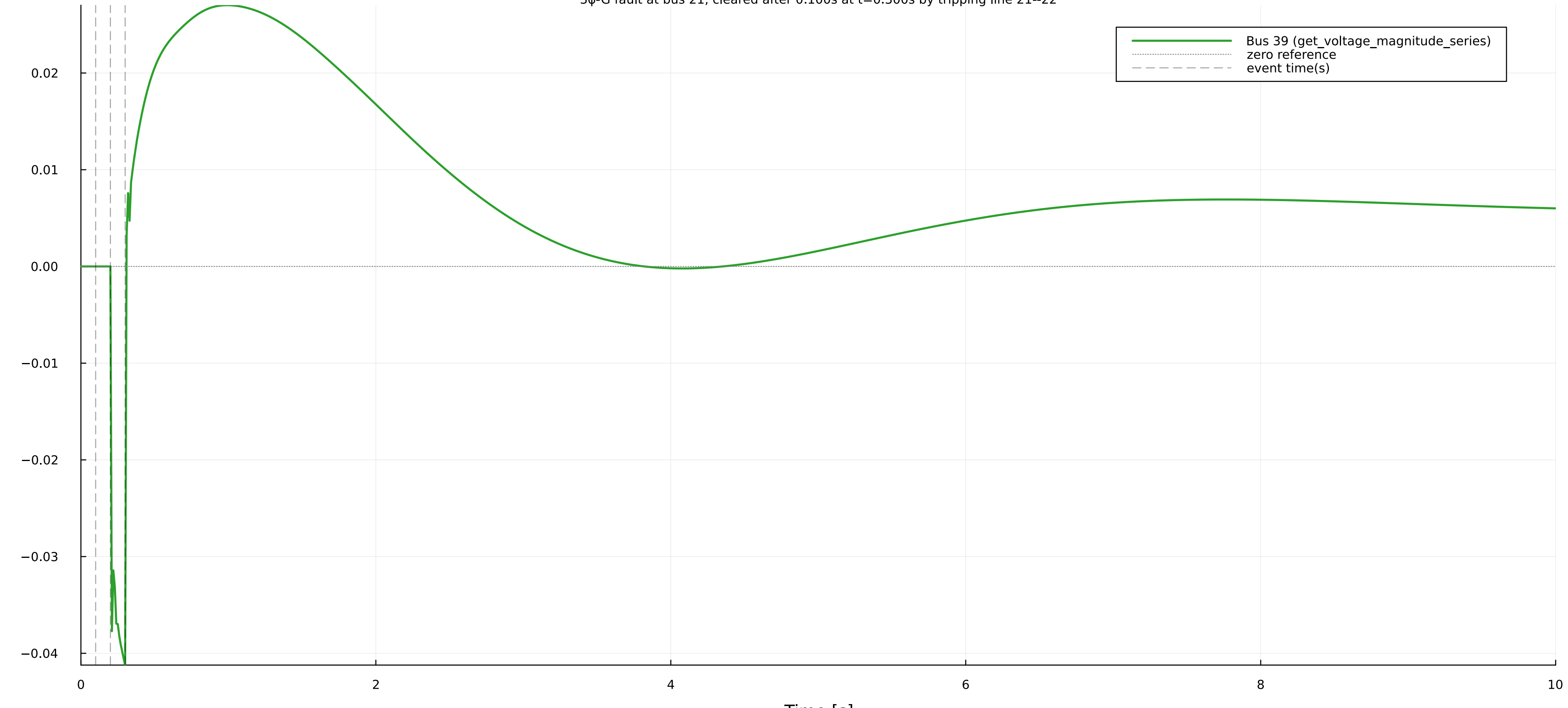
Voltage-magnitude deviation at bus 39 [V0=1.0300 pu] 3 \phi -G fault at bus 21, cleared after 0.100s at t=0.300s by tripping line 21--22
