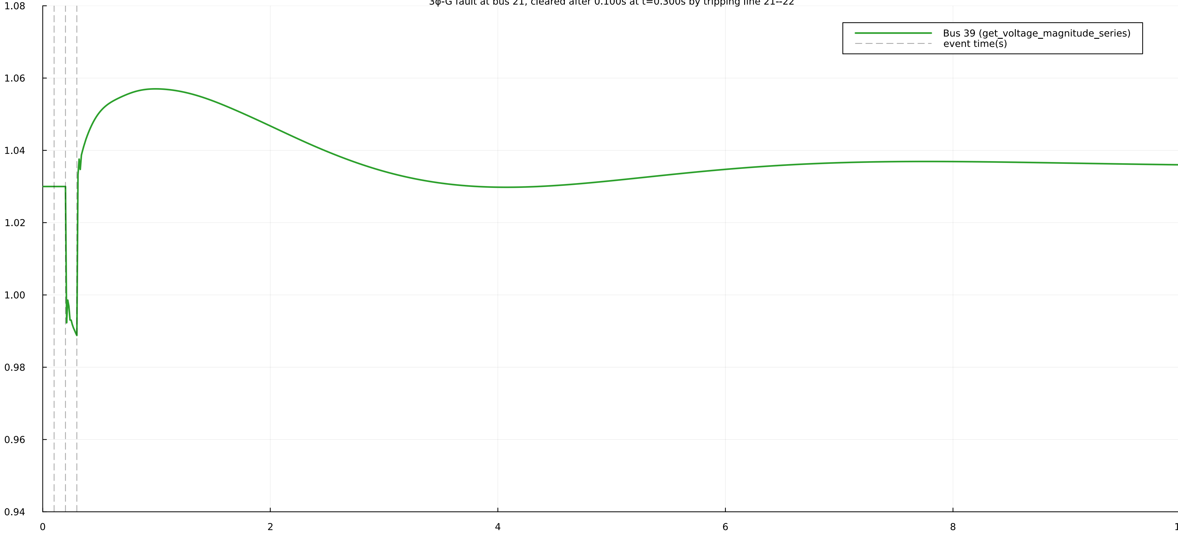
Voltage magnitude at bus 39 [V0=1.0300 pu] 3φ-G fault at bus 21, cleared after 0.100s at t=0.300s by tripping line 21--22
