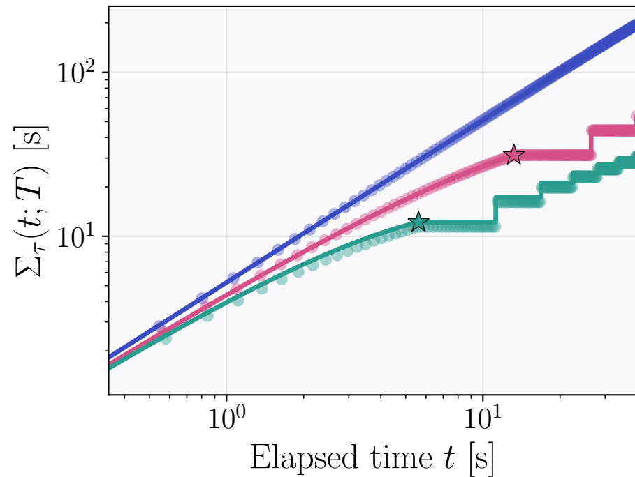
Steane
