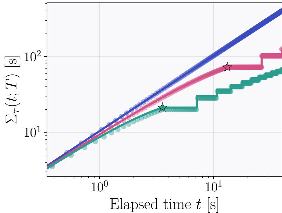
Shor
