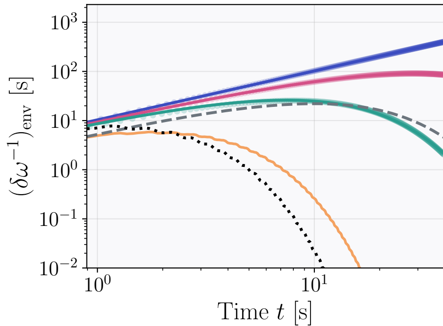
Shor
