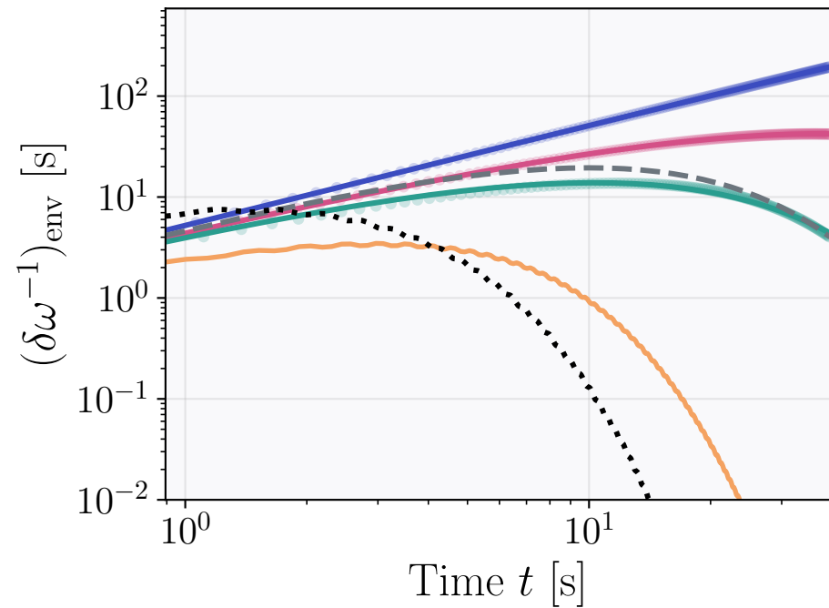
Steane
