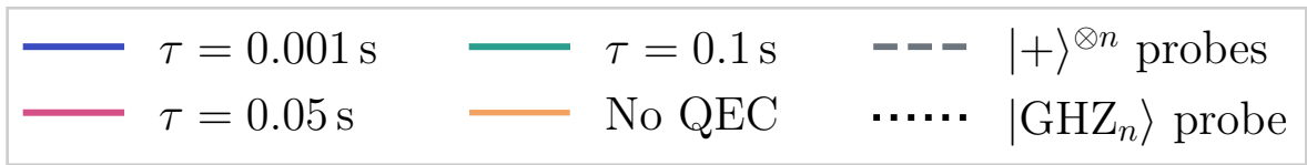
Steane
