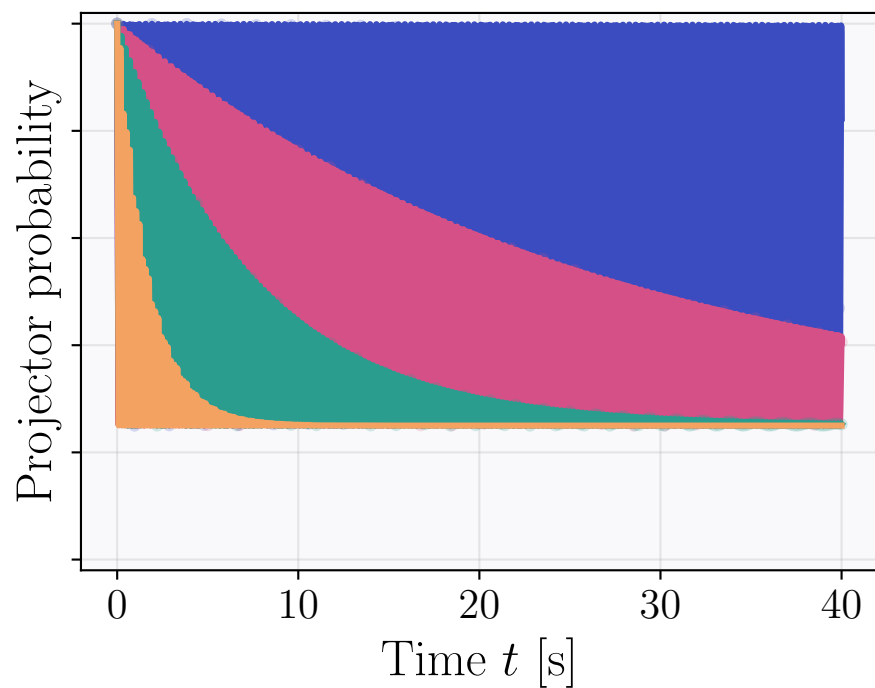
Shor
