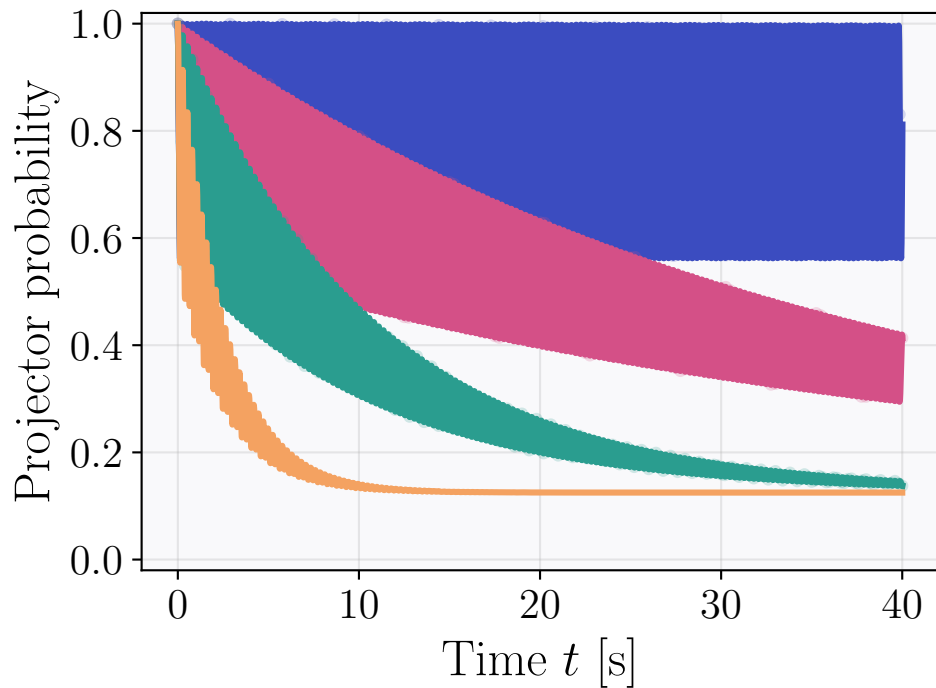
Steane
