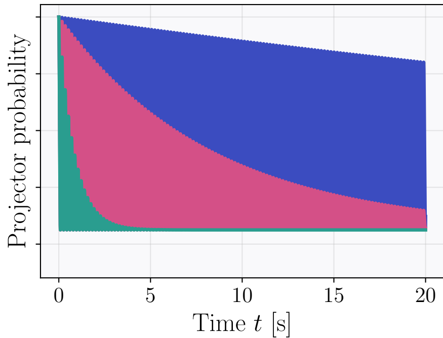
Shor
