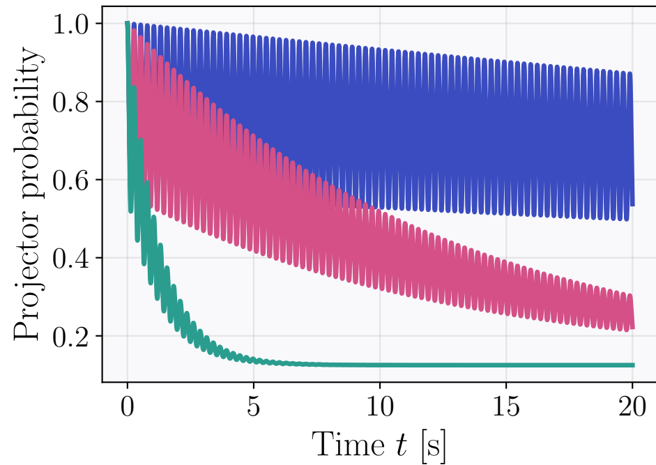
Steane
