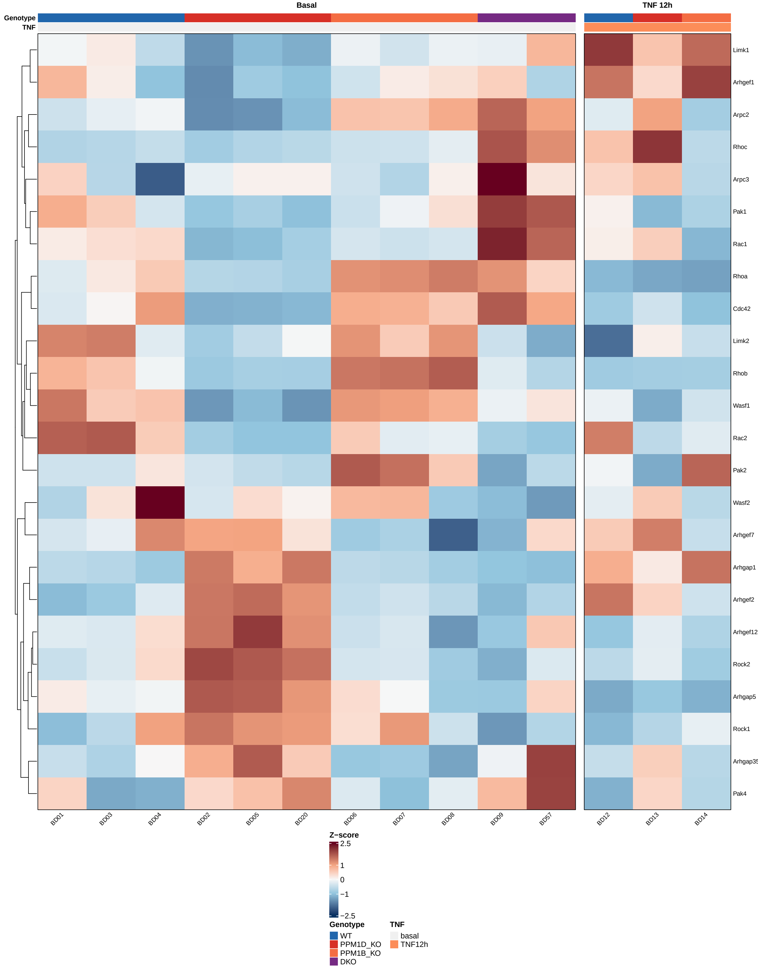
Rho GTPase network – 4 genotypes + TNF
