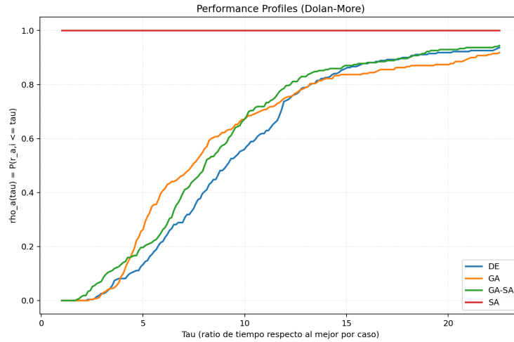
Figura 5: Performance profile de Dolan-Moré
