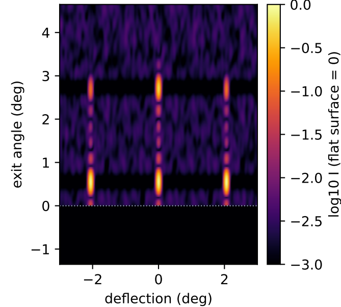
I_{00} = 0.0037
