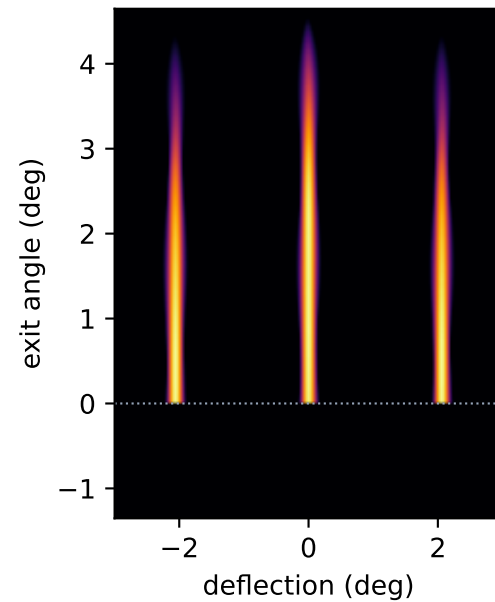
I_{00} = 0.8464
