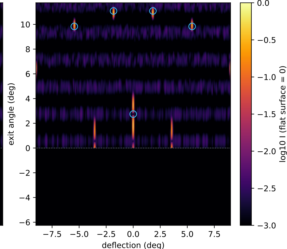
azimuth 30° — 5 reachable rods (-2,-3), (-1,-1), (00), (01) (13)
