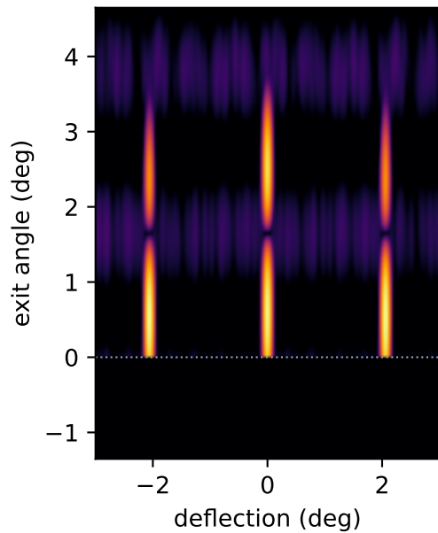
I_{00} = 0.0012
