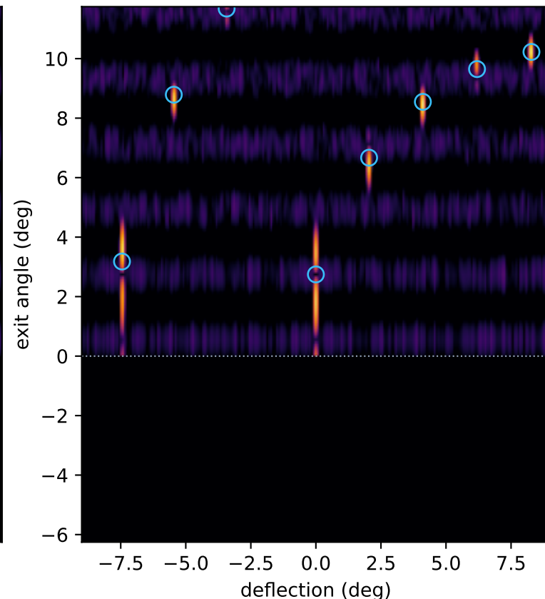
azimuth 10° — 8 reachable rods (-1,-4), (-1,-3), (-1,-2), (00) (01), (02), (03), (04)
