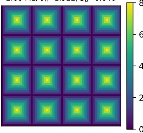
E periodic pyramid array 2.66 ML, \sigma_h=1.922 , S_d=0.646
