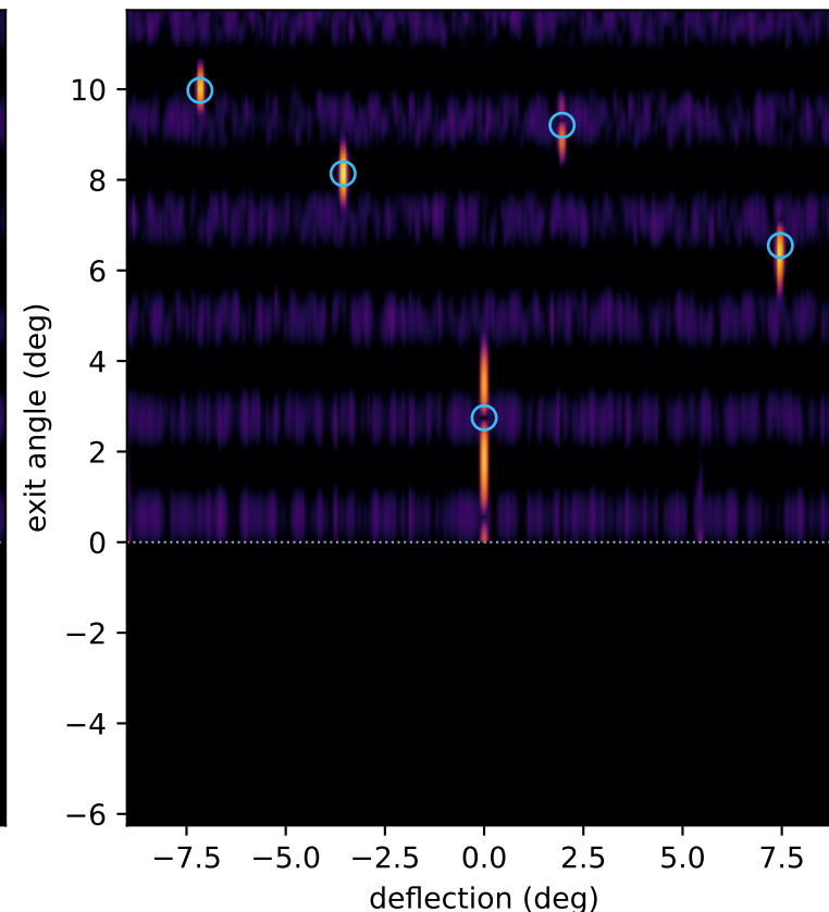
azimuth 20° — 5 reachable rods (-2,-4), (-1,-2), (00), (01) (14)
