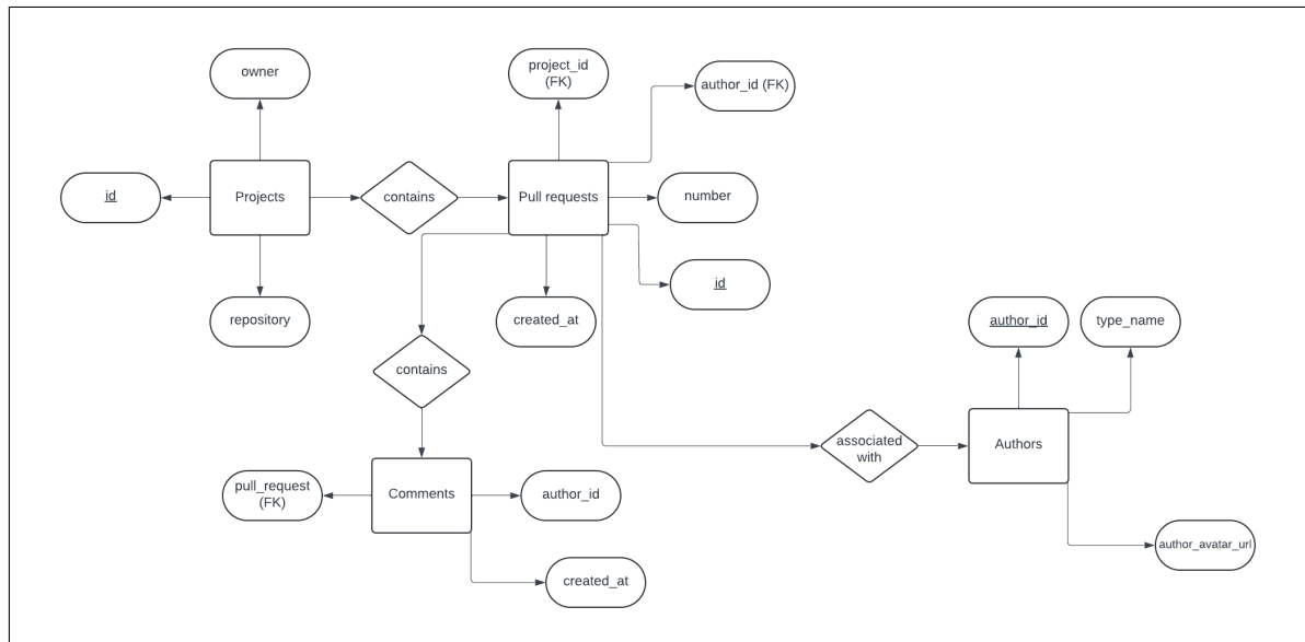
Figure 2.1: ER diagram of final database schema.
