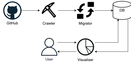
Figure 1: Overall framework
