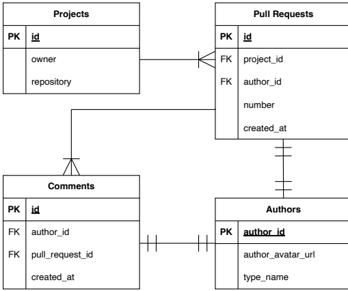
Figure 2: Entity Relationship Diagram
