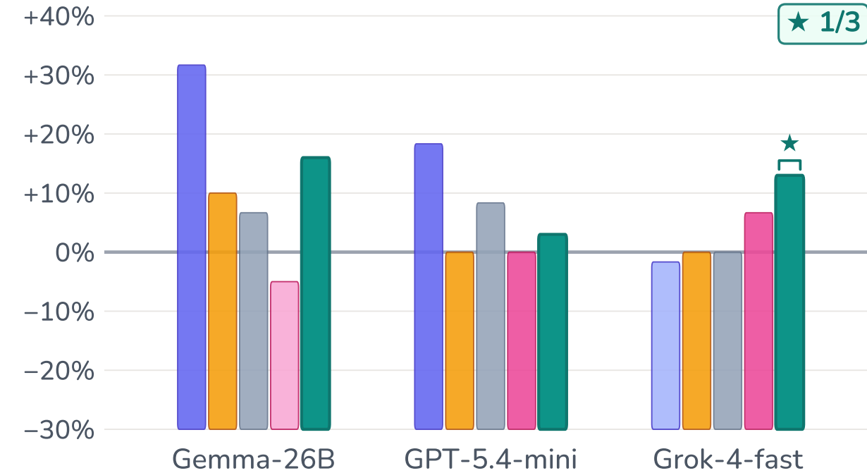
ScienceWorld
