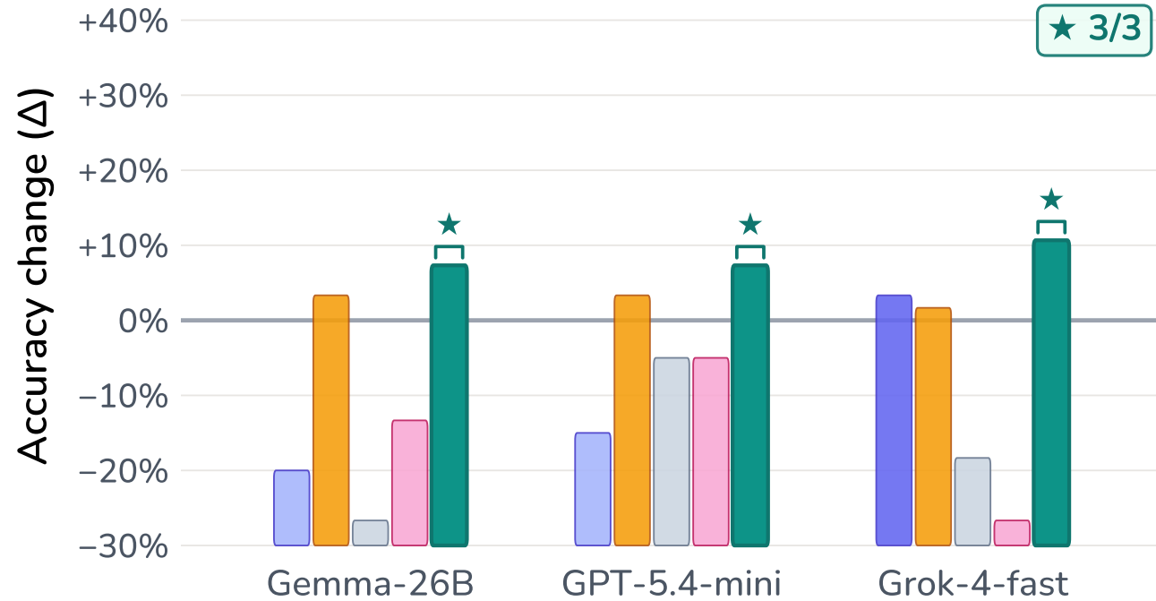
ALFWorld (IOD)
