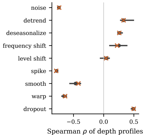
(a) L3: 9/9 replicate
