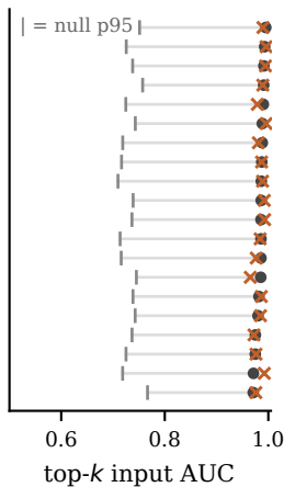
(b) transfer: 20/20
