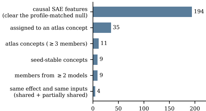
(a) concept candidates per evidence rung
