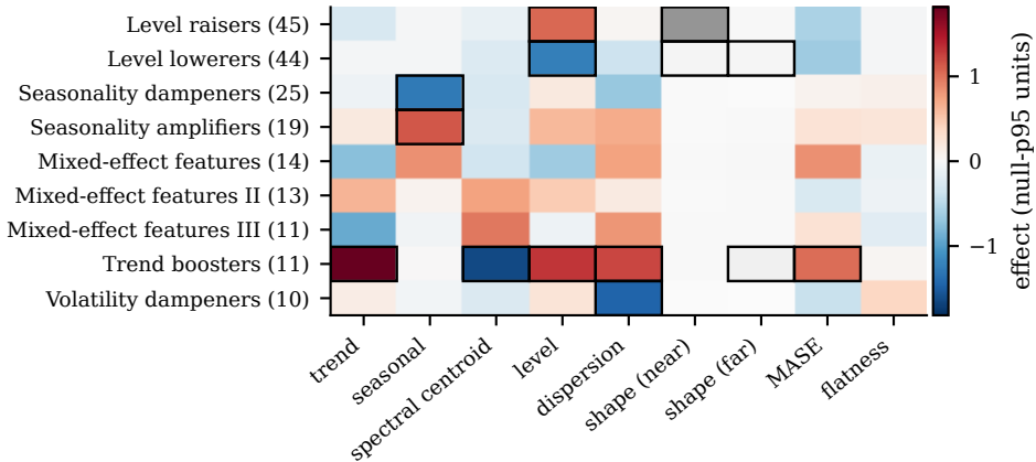
(a) what each family does (boxed: clears null)
