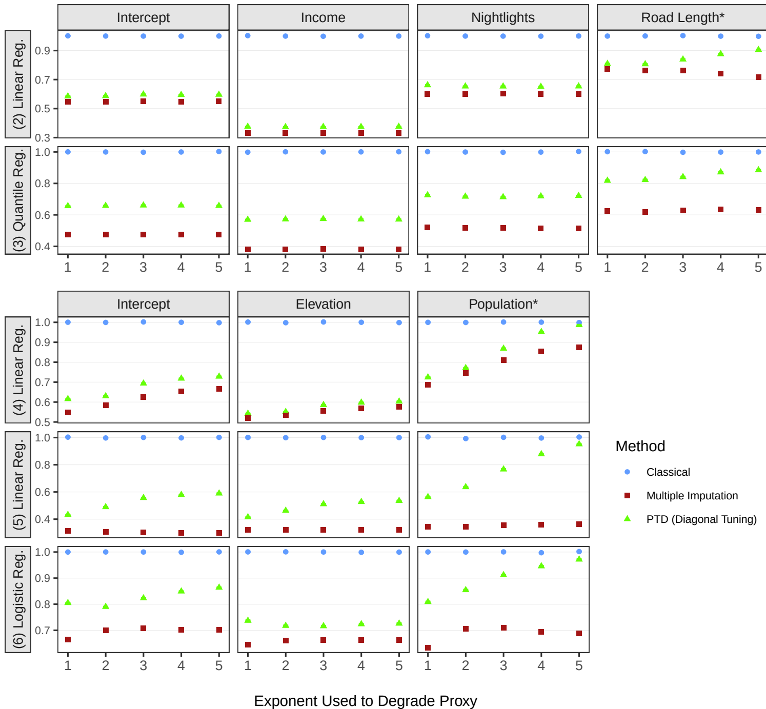
Normalized Mean Confidence Interval Width
