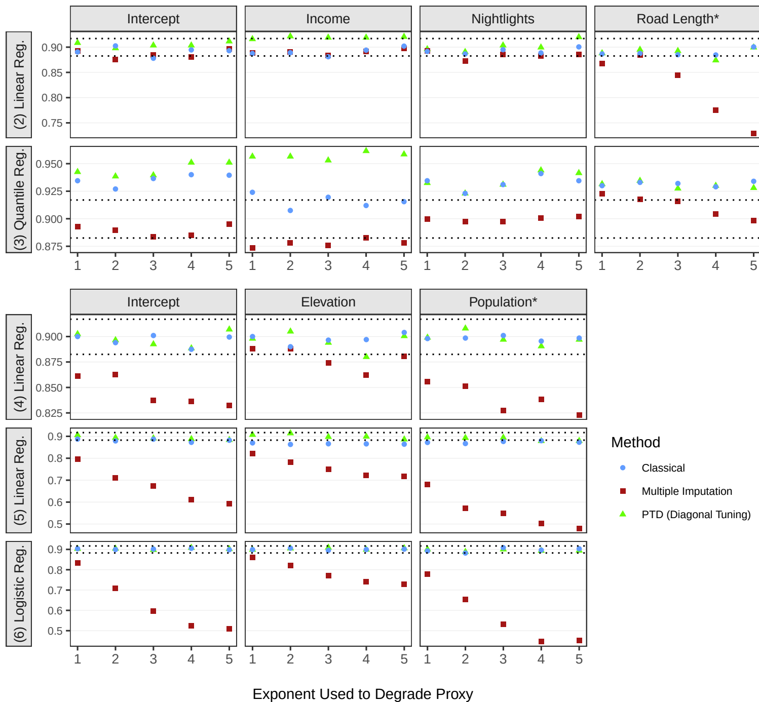
Empirical Coverage
