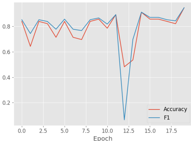
Fig. 6: Evolution of the accuracy and F1 score during training
