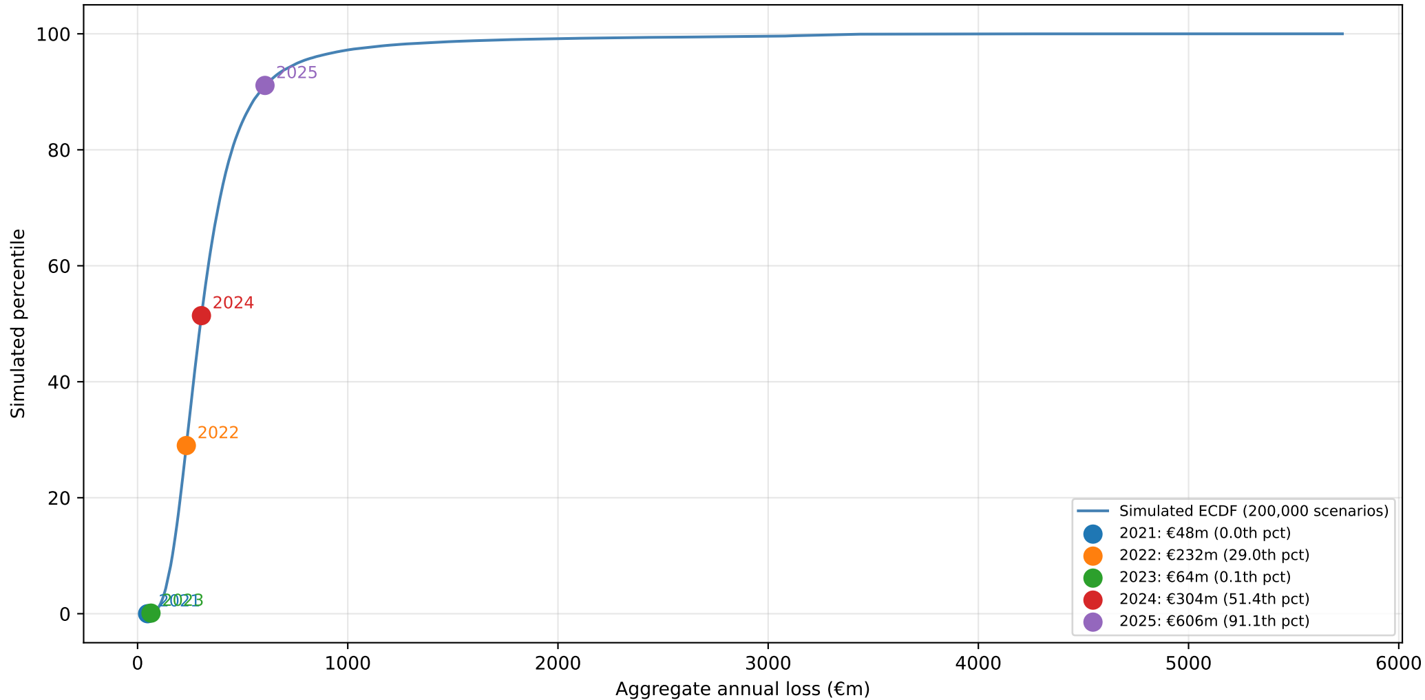
Backtest: holdout years (2021–2025) against the Phase 3 simulated distribution (model fitted on 2009–2020 PRDF training data only)
