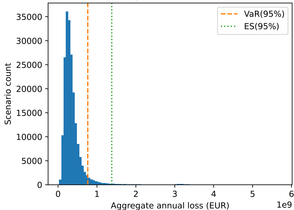
Simulated portfolio loss distribution
