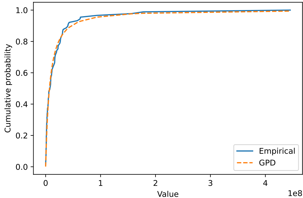
GPD tail vs empirical (exceedances over EUR 5.8m)
