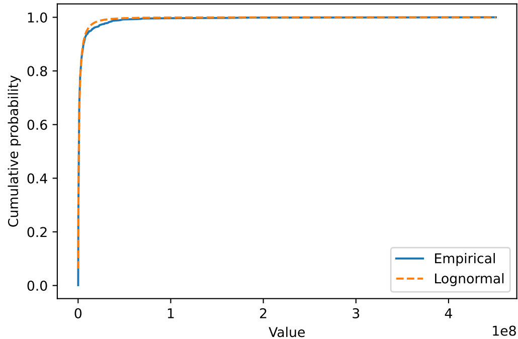
Lognormal body vs empirical (full sample)
