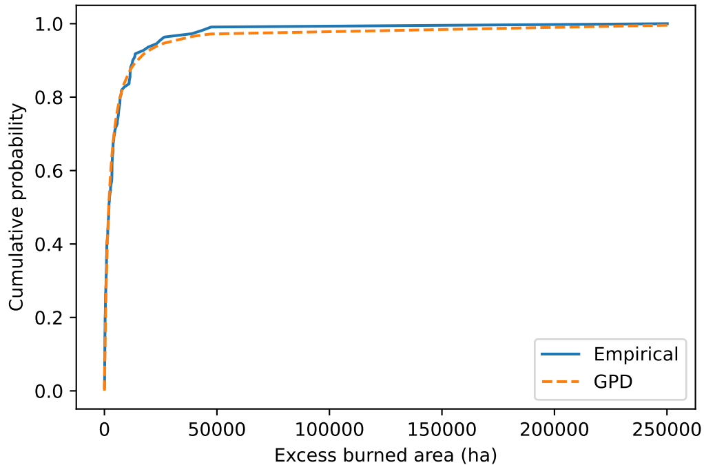
GPD tail vs empirical (exceedances over 2,058 ha)
