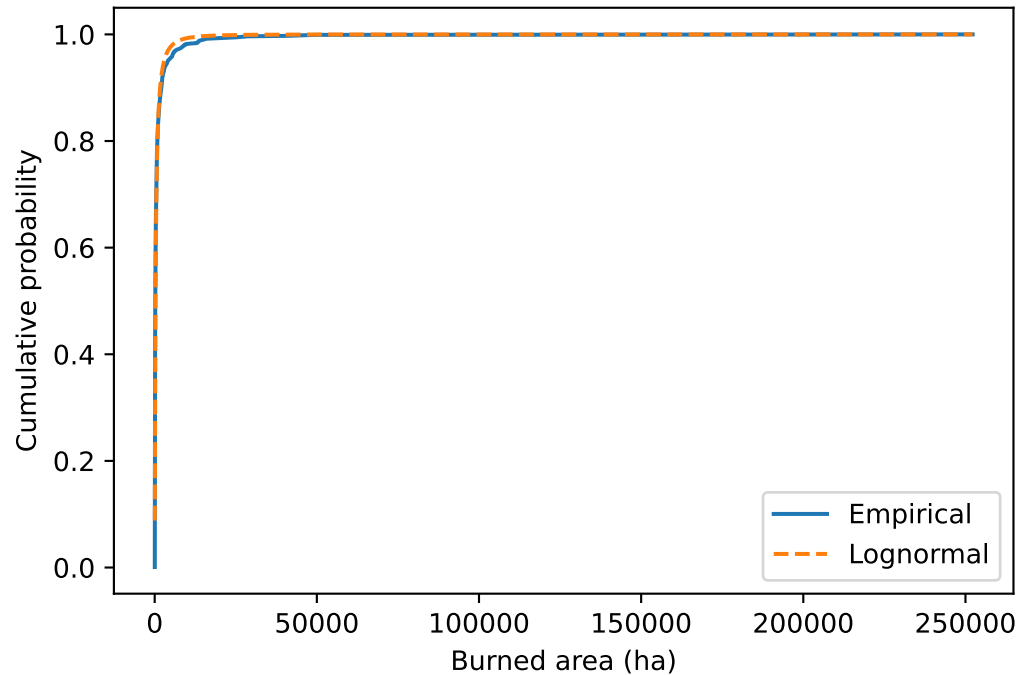
Lognormal body vs empirical (full sample)
