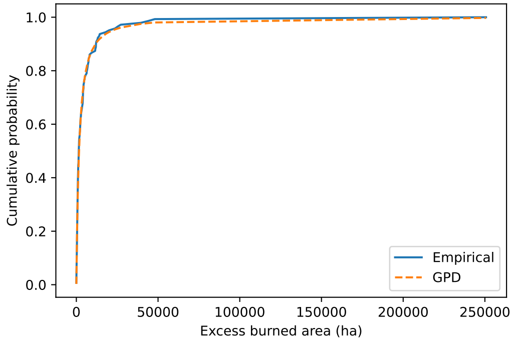
GPD tail vs empirical (exceedances over 1,490 ha)
