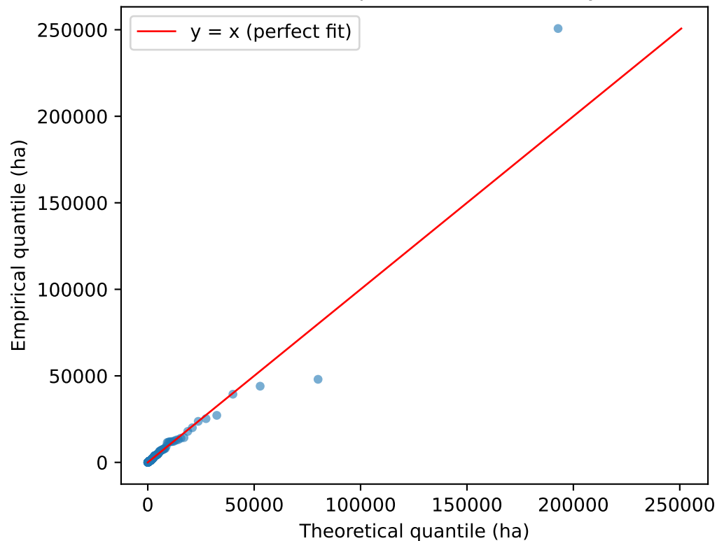
GPD tail QQ (top 13% of events, vs y=x )
