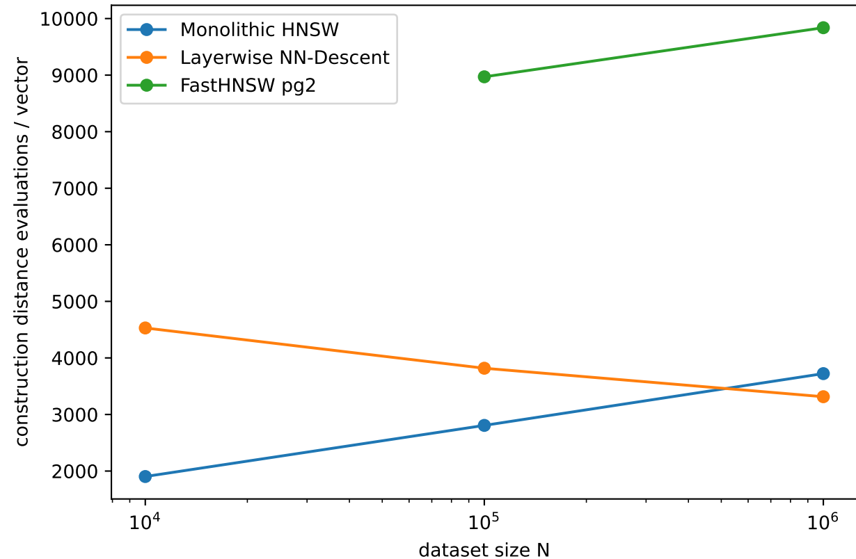
Canonical constructor distance cost per input vector
