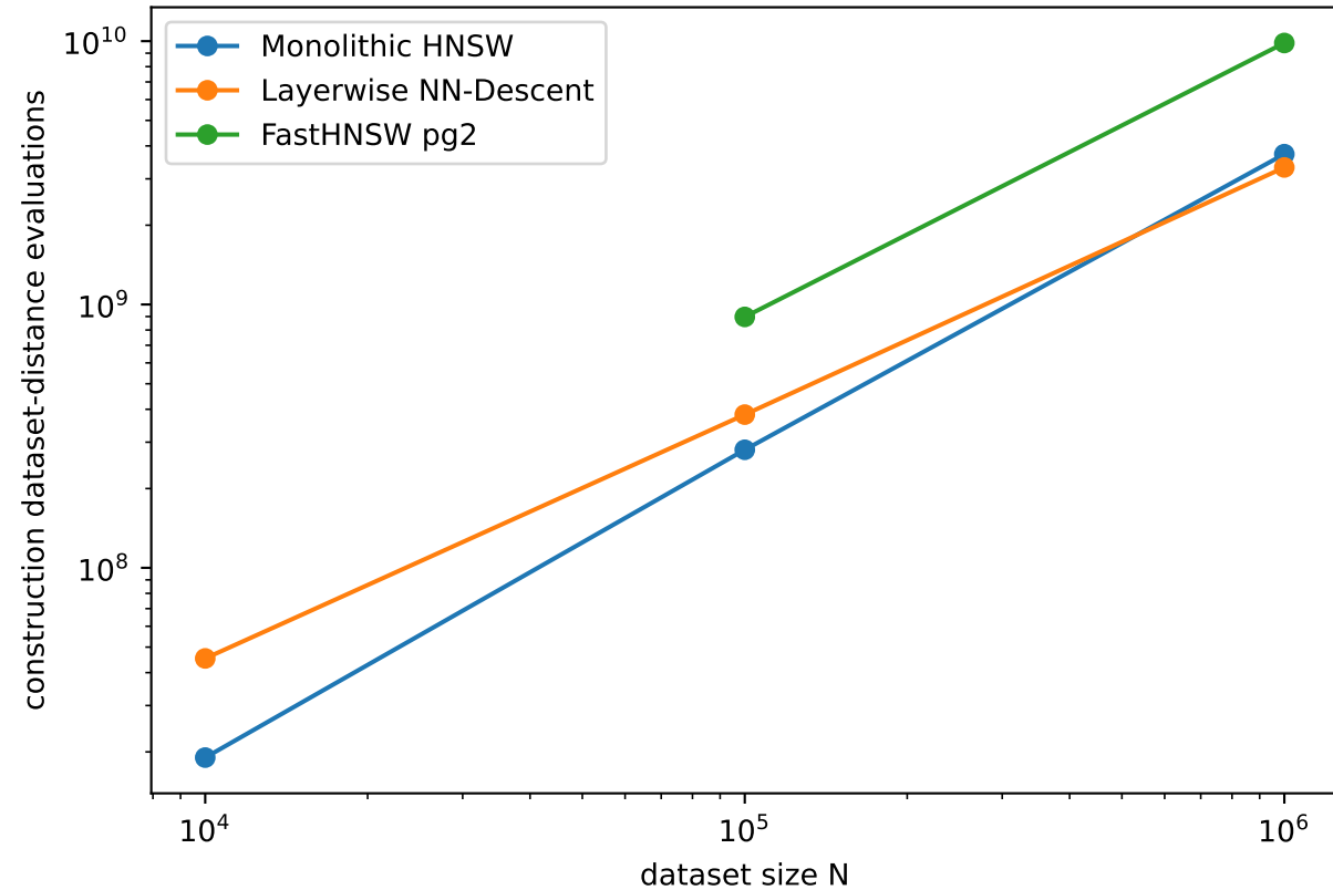
Canonical constructor distance cost vs dataset size
