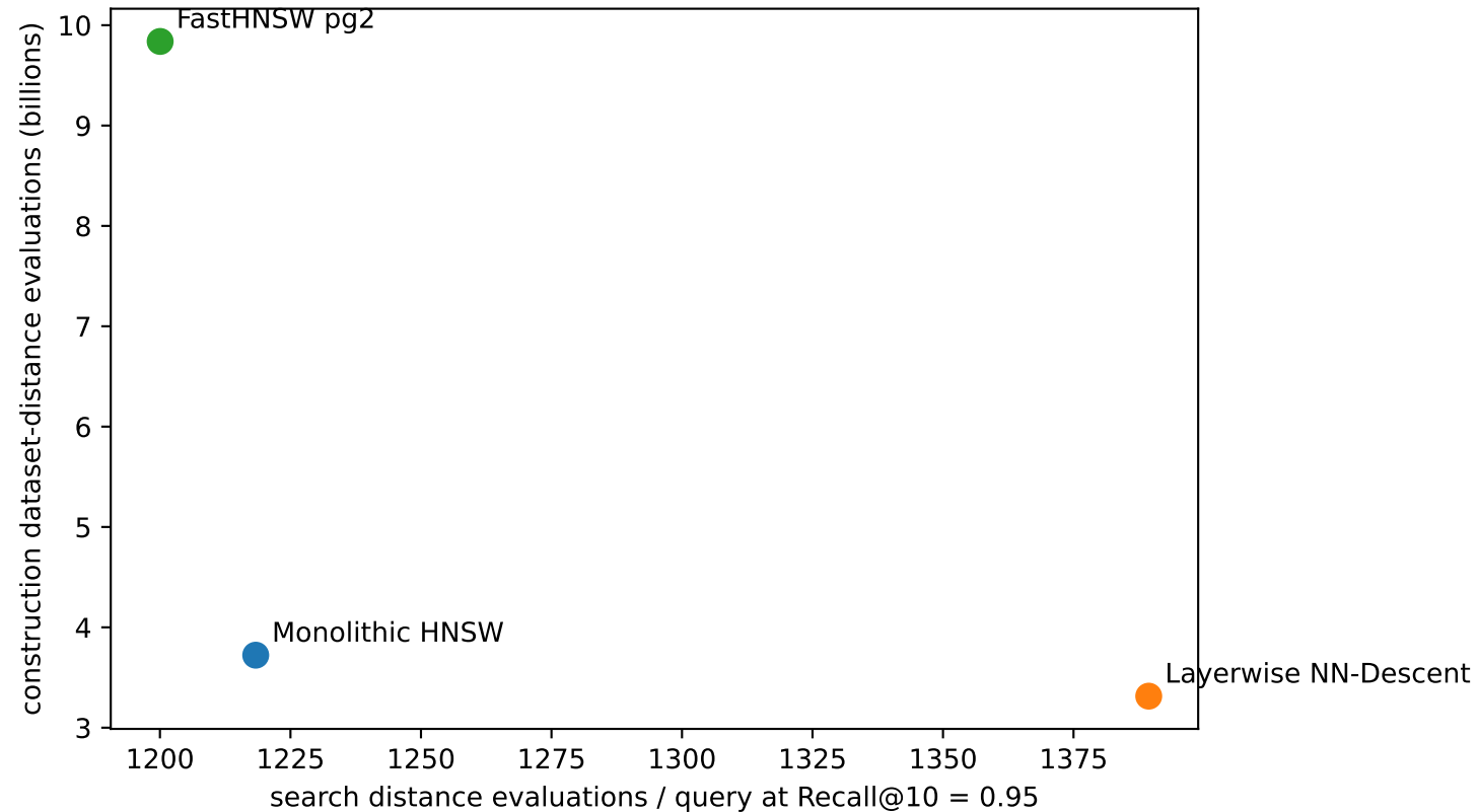
1M construction/search-distance trade-off
