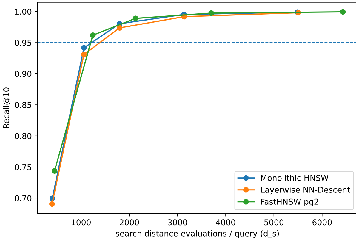
1M search quality vs counted search distance
