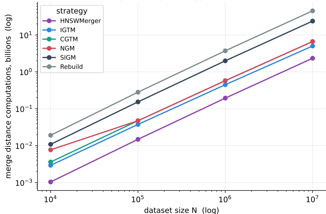
Merge cost by strategy across scale
