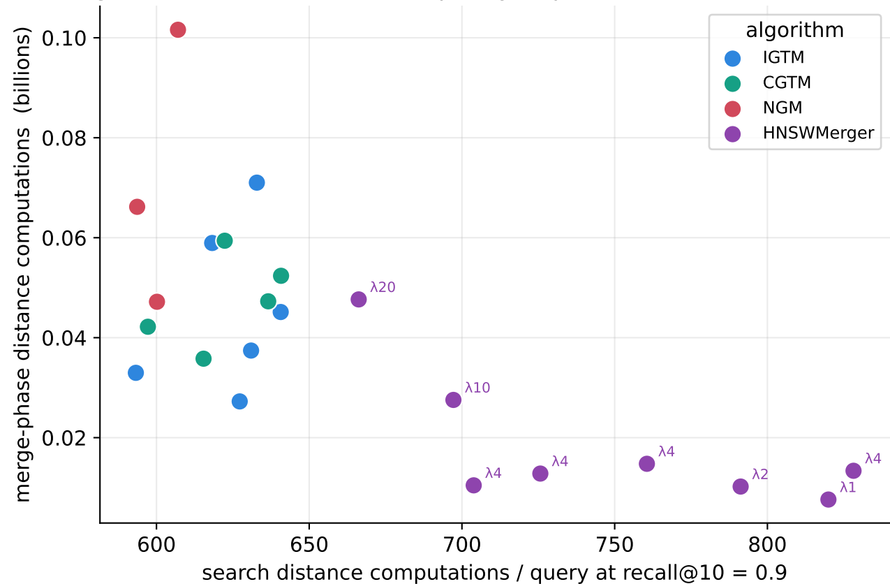
Merge cost at matched search quality, 2 partitions (SIFT 100K (BIGANN))
