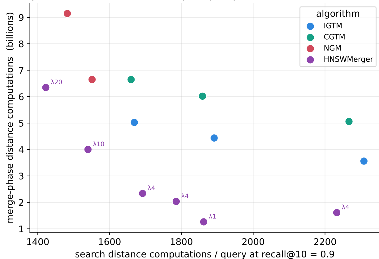
Merge cost at matched search quality, 2 partitions (SIFT 10M (BIGANN))
