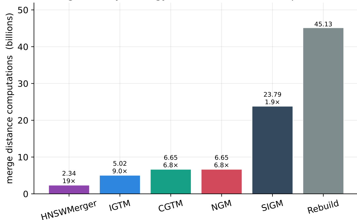
Merge cost by strategy (SIFT 10M (BIGANN), 2 partitions)
