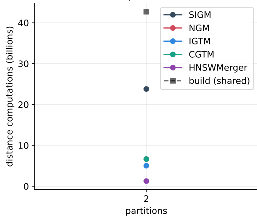
Cost vs partition count
