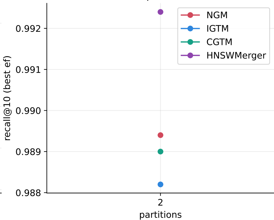
Recall vs partition count
