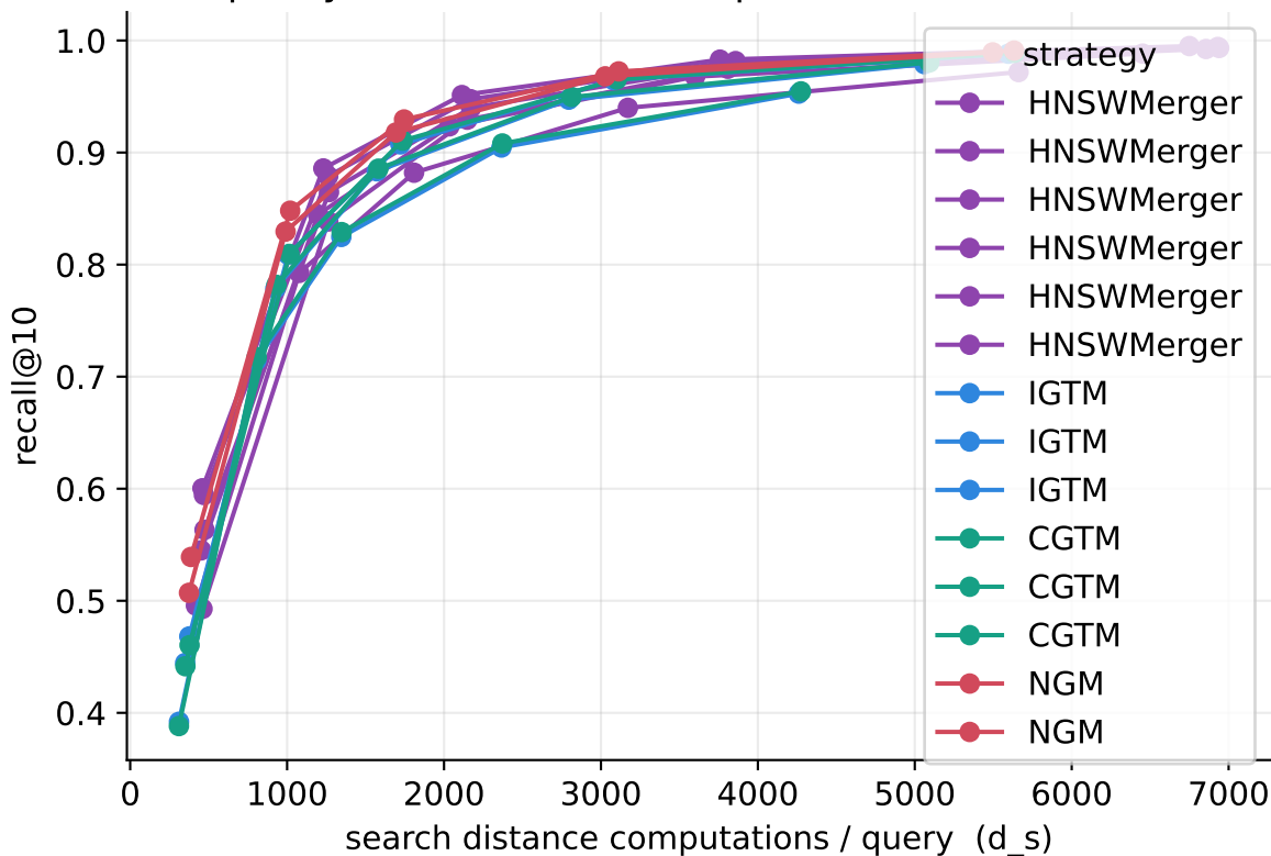
Search quality vs search cost at 2 partitions (SIFT 10M (BIGANN))
