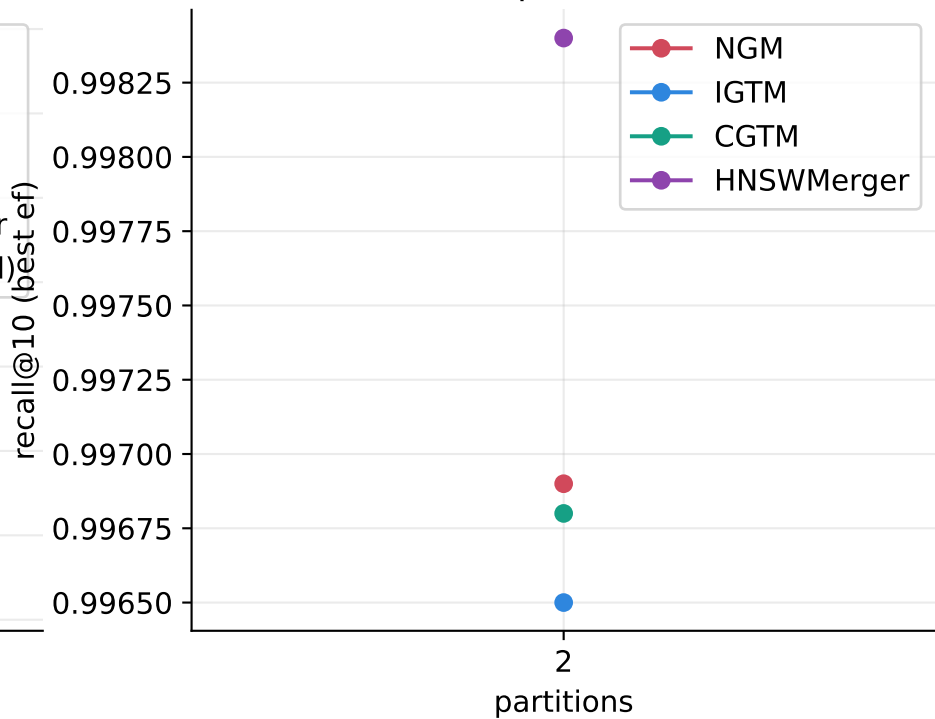
Recall vs partition count
