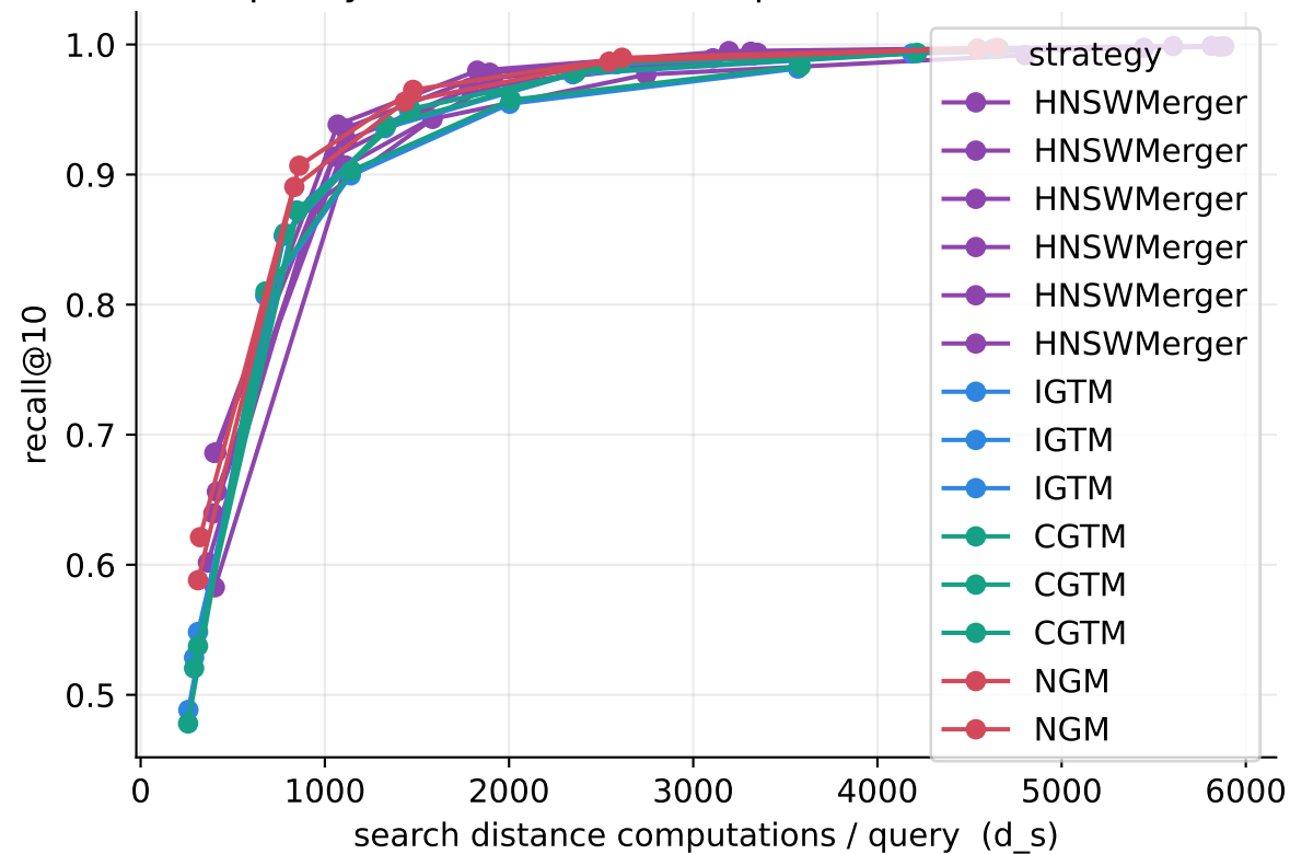
Search quality vs search cost at 2 partitions (SIFT 1M (BIGANN))
