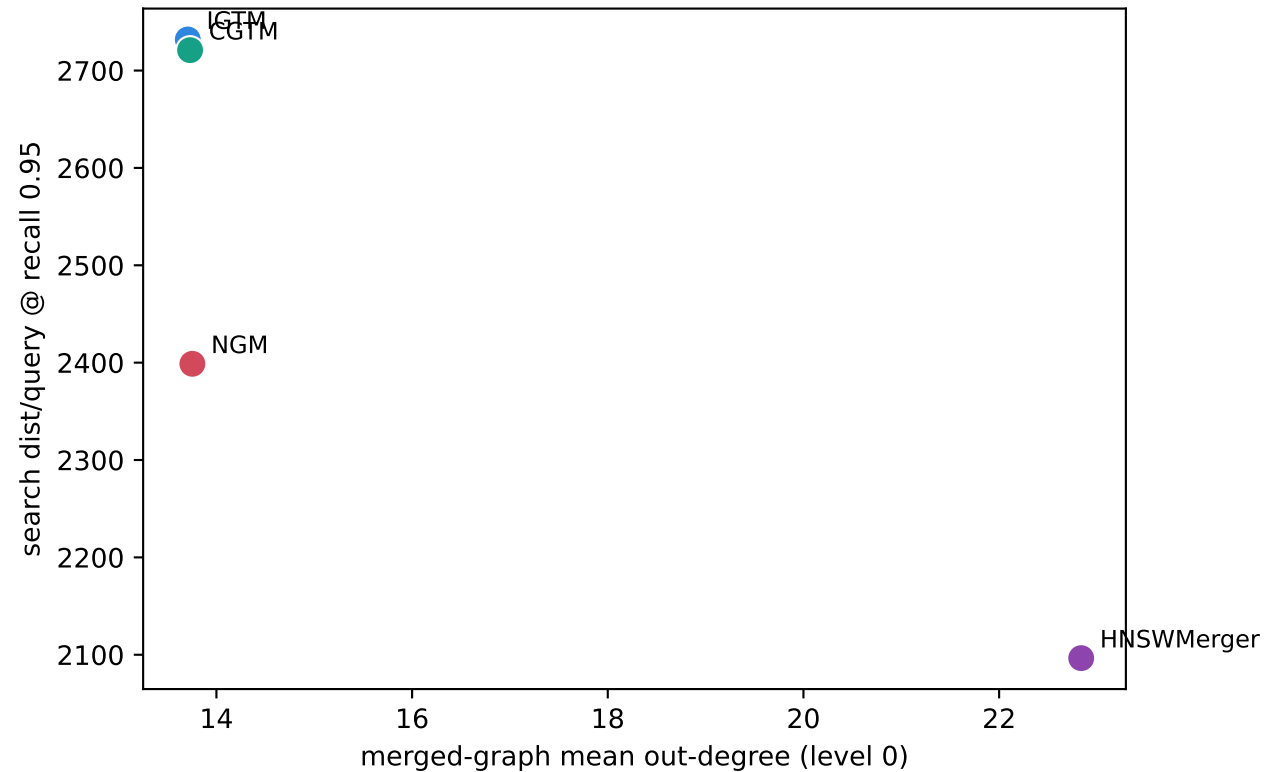
Graph density vs search cost (N=10,000,000)
