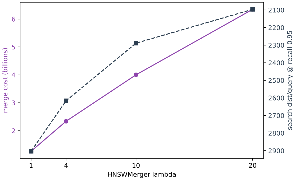
HNSWMerger lambda: cost vs search quality (N=10,000,000)
