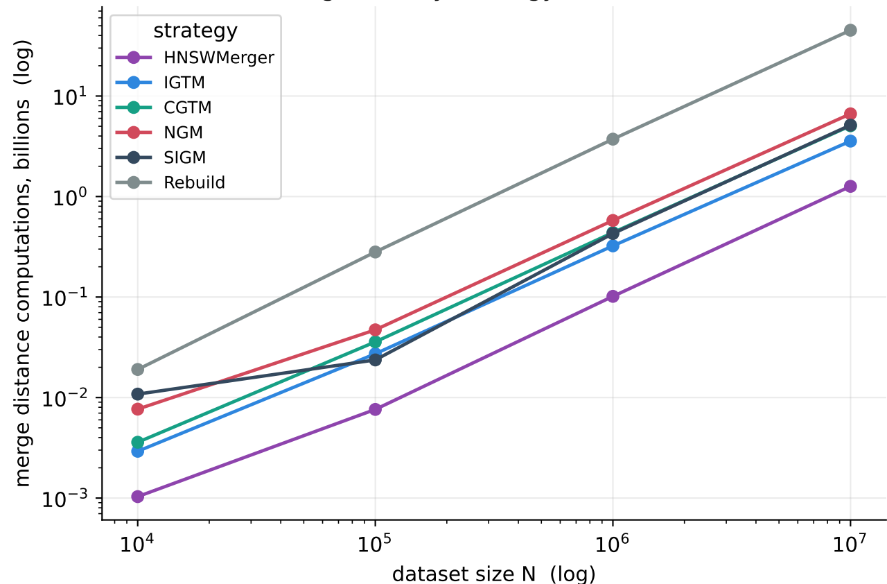
Merge cost by strategy across scale
